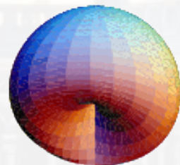
cross surface
