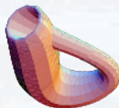
Klein bottle
